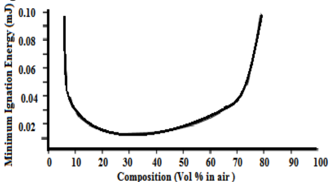
Figure 1. Minimum ignition energy of hydrogen in air [18]
