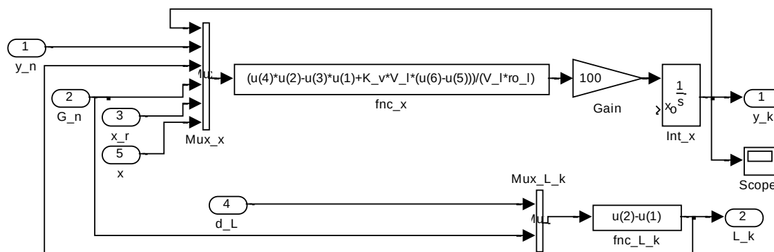
Figure 11. Volatile component concentration change computer model of the gas phase quasi-apparatus processes in the third stage of the oil deodorization facility and computer model of the gas consumption quasi-apparatus process.
