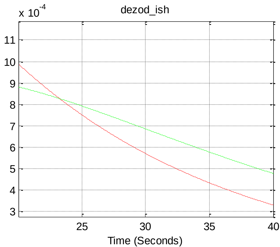
Figure 16. Consumption of volatile components passing into the gas phase. Concentration of volatile components in oil (red line) and gas phase
